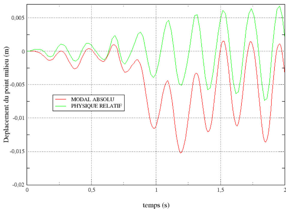
Illustration 3: SDLL302b : calcul multi-appui
