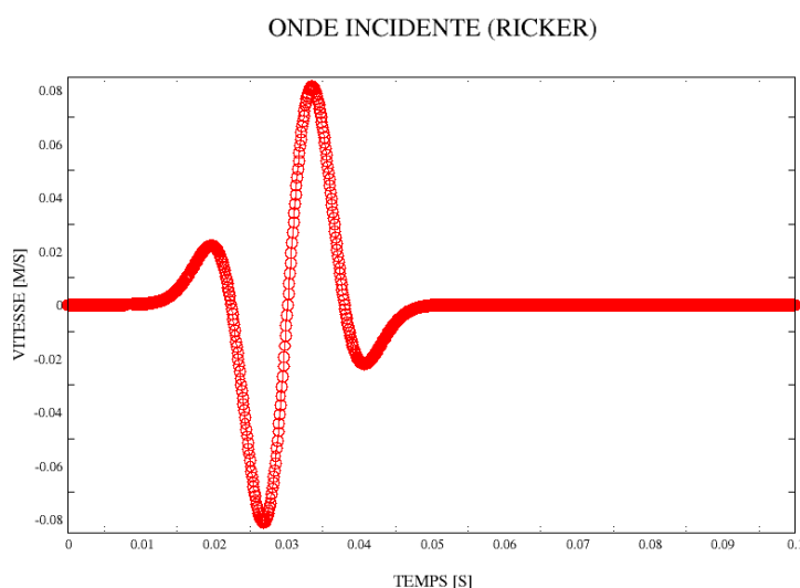
Image 1.4.1 : Ondelette incidente (Ricker)
