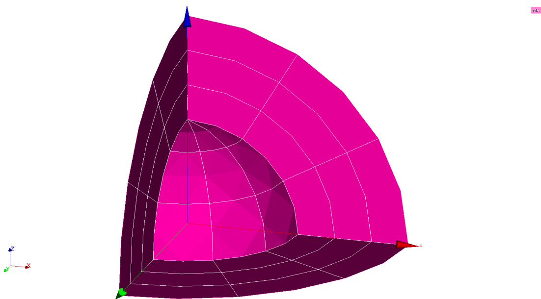
Figure 4.2-a: Maillage 3D quadratique
