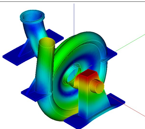
Illustration 7: Mode 3 du calcul modal direct
