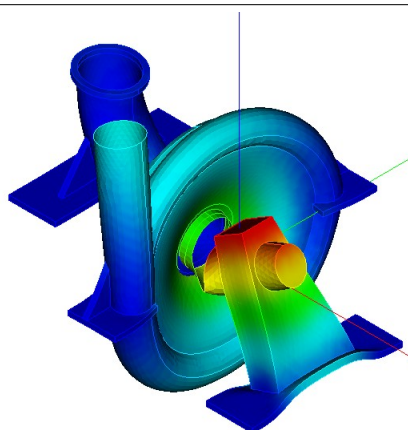
Illustration 11: Mode 2 du calcul modal direct
