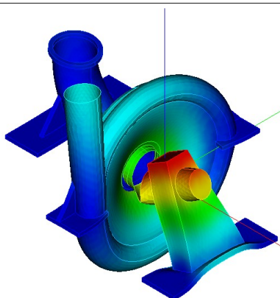
Illustration 5: Mode 2 du calcul modal direct
