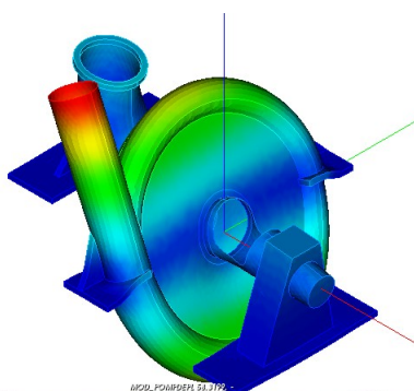
Illustration 3: Mode 1 du calcul modal direct
