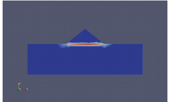
Illustration 3: REAC_NODA / GROUP_MA=('BARRAGE','DE')
