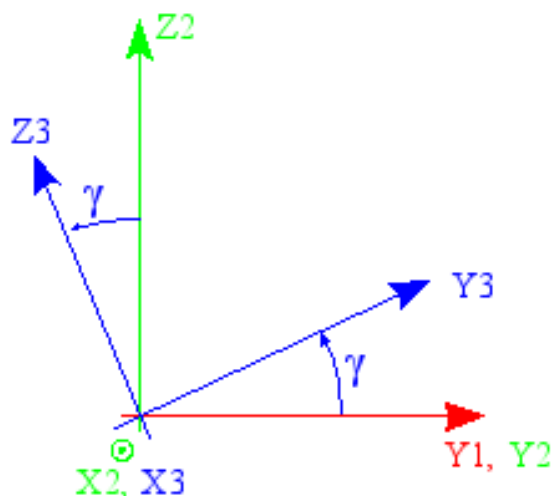
Figure 3.9.3-3 : angle \gamma .
