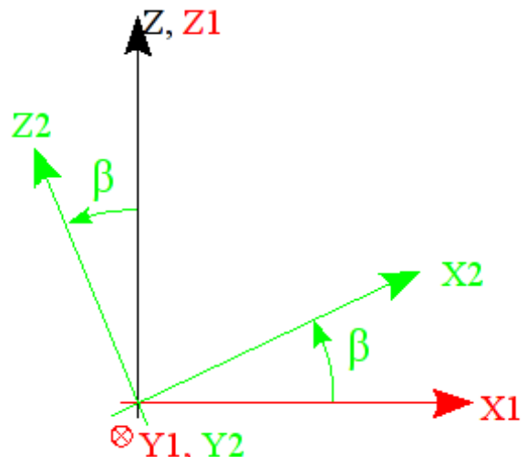
Figure 10.4-2 : angle \beta .
