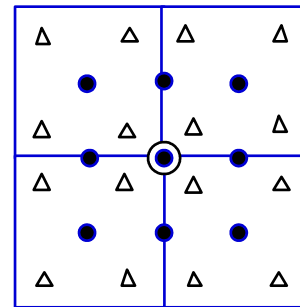
QUAD9
