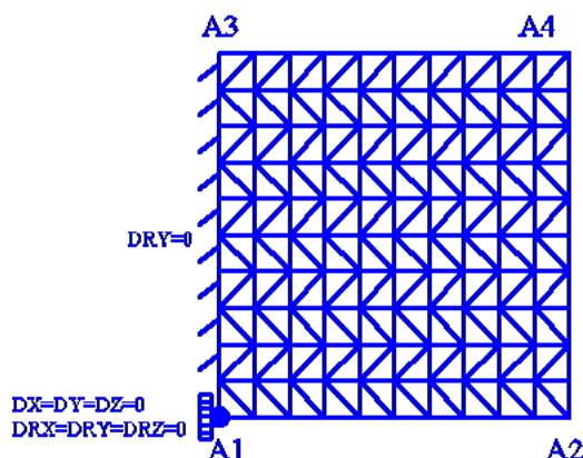
Figure 7.1-a: maillage
