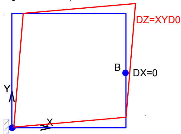
Figure 16.1-b : Conditions aux limites
