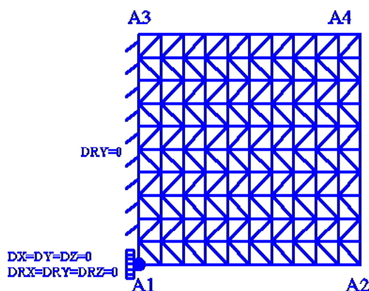
Figure 15.1-a: maillage
