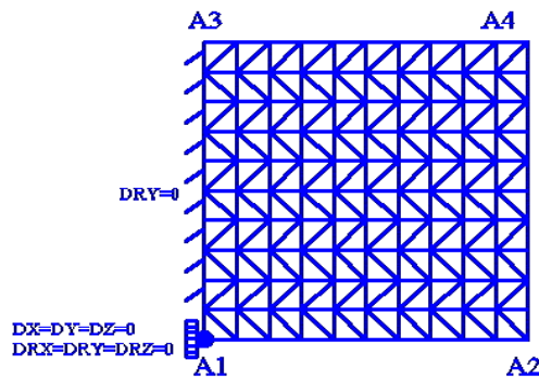
Figure 16.1-a: maillage
