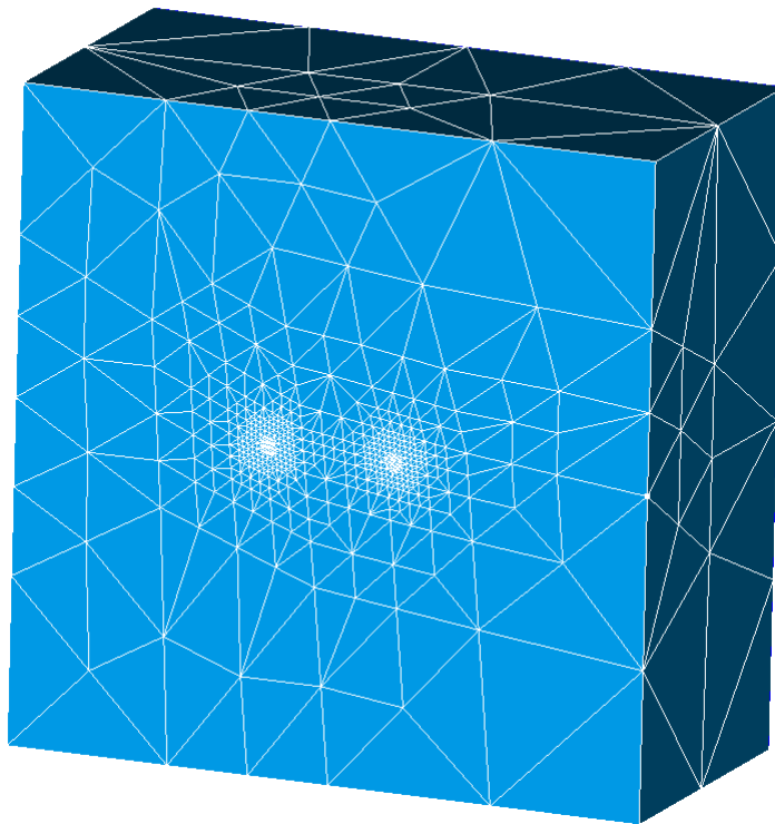
Figure 4.1: maillage raffiné de la structure
