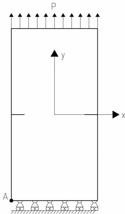
Figure 1.3-a: conditions aux limites et chargements
