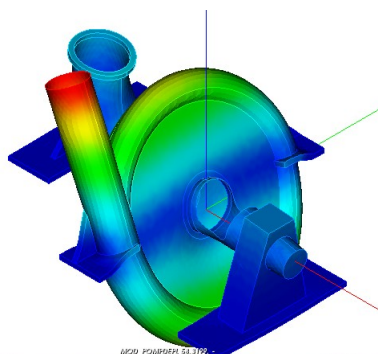
Illustration 9: Mode 1 du calcul modal direct
