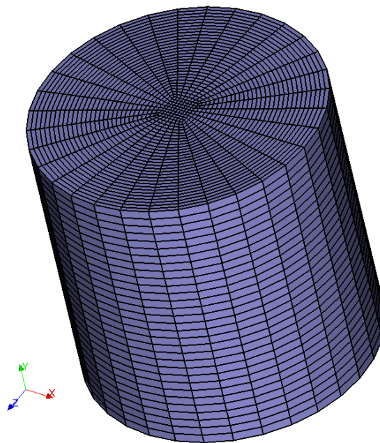
Figure 6.2-1: Maillage D
