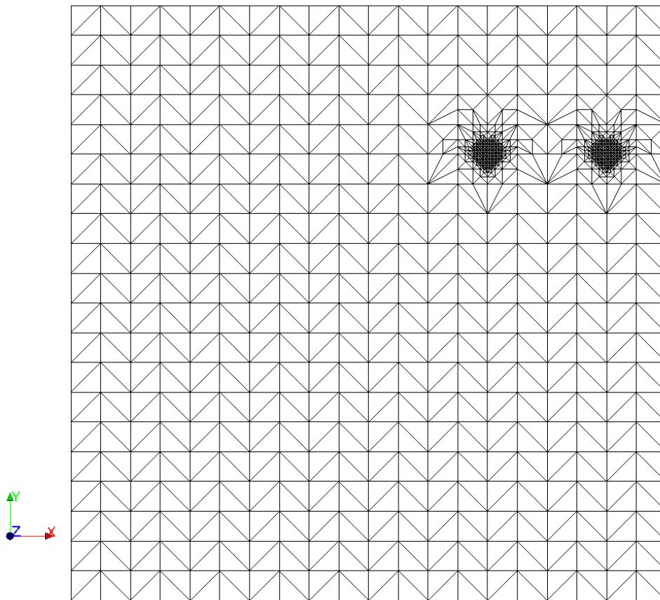
Figure 5.2-1: maillage sain raffiné
