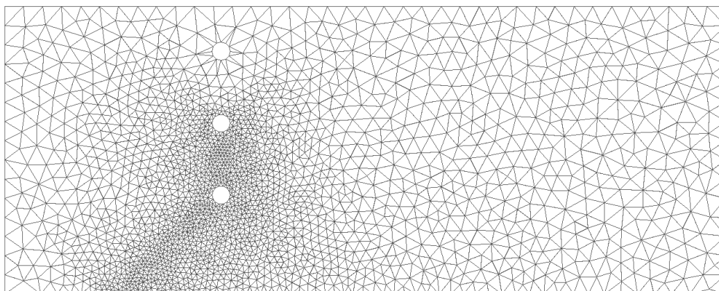
Figure 3.2-a: maillage de la structure
