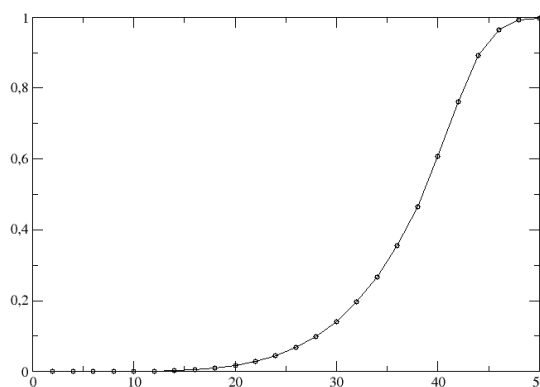
Proba. rupture Weibull- Eprouvette CT
