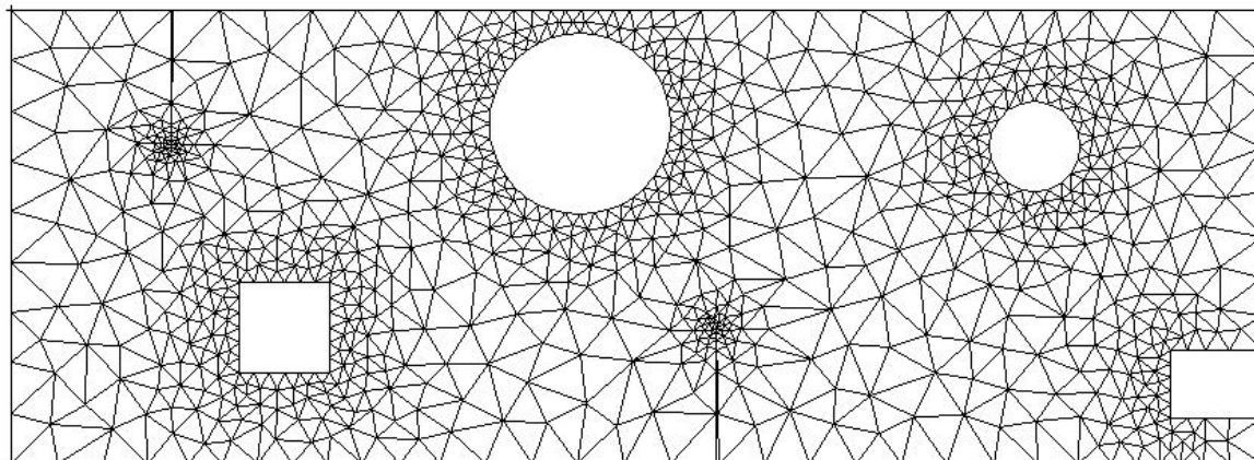
Figure 5.4-c : Maillage initial
